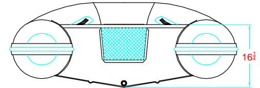
AFT VIEW VISTA TRASERA
